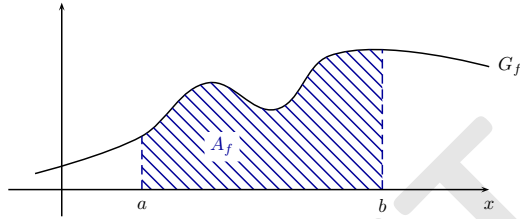
FIGURE 6.5: Geometric interpretation of the Riemann integral.
