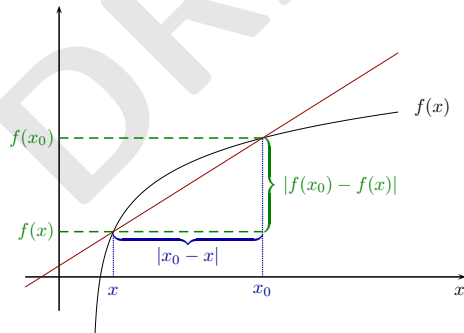
FIGURE 6.1: Geometric interpretation of the difference quotient in the case \mathbb{F} = Y = \mathbb{R} : The difference quotient \frac{f(x) - f(x_0)}{x - x_0} is the slope of the secant of the graph of f through the points (x_0, f(x_0)) and (x, f(x)) . For x \rightarrow x_0 the secant becomes the tangent of the graph of f in the point (x_0, f(x_0)) ; f'(x_0) is the slope of the tangent.
