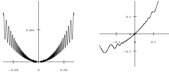
FIGURE 6.2: The function f(x) = x^2(1 + (\sin x^{-1})^2) in the left picture has a global isolated minimum at 0 but there is no right neighbourhood J of f such that f|_J is monotonically increasing. The function g(x) = x + 2x^2(1 + (\sin x^{-1})^2) in the right picture has derivative g'(0) = 1 but it is not monotonic locally at 0.
