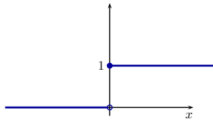
Example 5.2 (vii): Heaviside function
