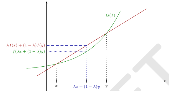
FIGURE 6.4: Convex function: f(\lambda x + (1 - \lambda)y) \leq \lambda f(x) + (1 - \lambda)f(y) for all x < y in the domain of f :
