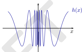
h(x) = \sin(x^{-1}) (Exercise 10.1)
