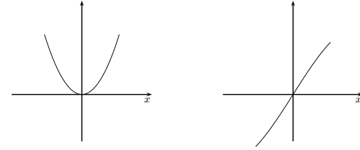
FIGURE 6.3: If f looks like the function on the left, then its derivative looks like the function on the right and vice versa.
