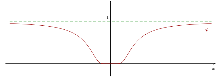
FIGURE 7.1: The non-analytic C^\infty function \varphi (see Theorem 7.18). Although the plot gives another impression, \varphi has an isolated global minimum at 0.
