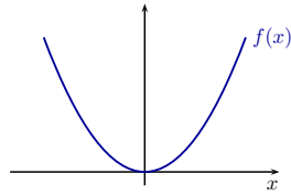
Example 5.2 (vi): f(x) = x^2
