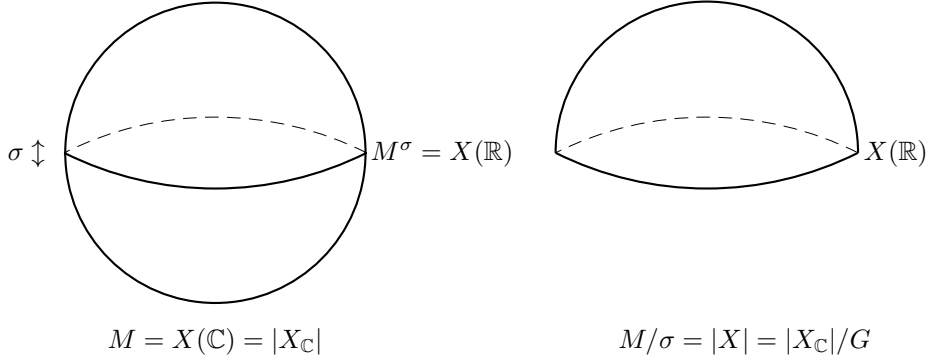
FIGURE 1. X = \mathbb{P}_{\mathbb{R}}^1 = \text{Proj}(\mathbb{R}[X_0, X_1])
